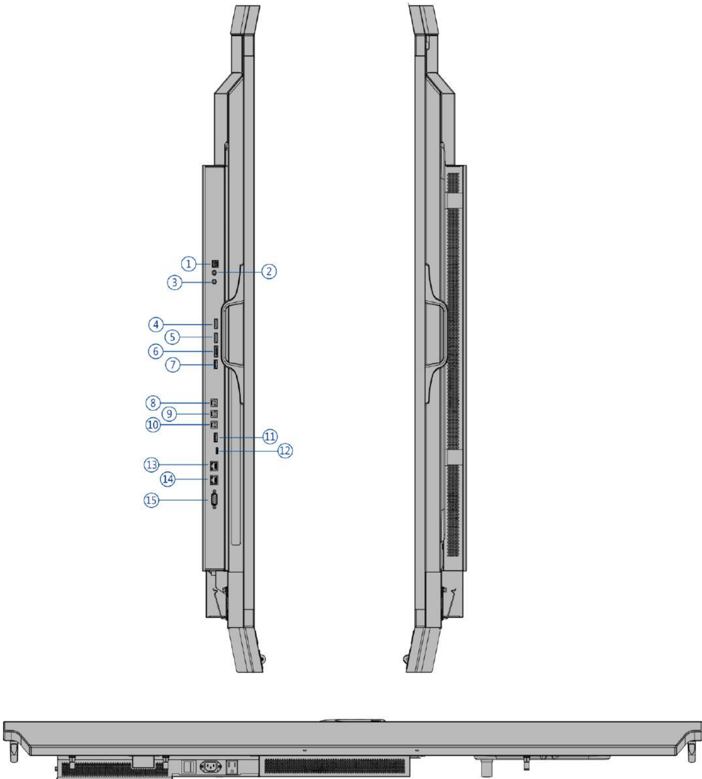
Figure 2-2. Display Input Panel View
