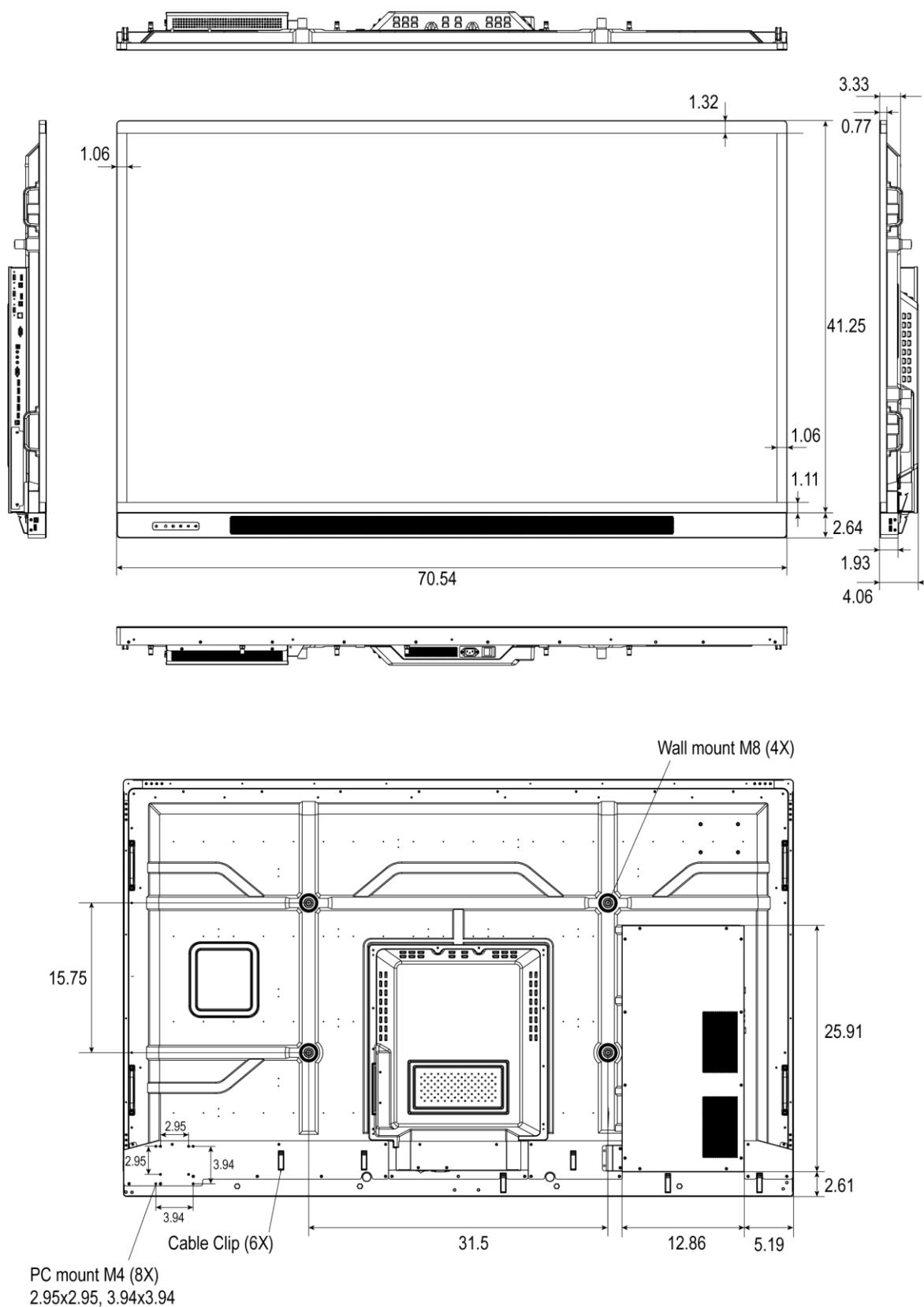
Figure 7-1. AVF-7550 Display Dimensions (inch)
